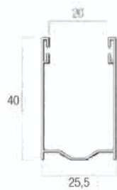
Guida in alluminio GUIAL40x25
